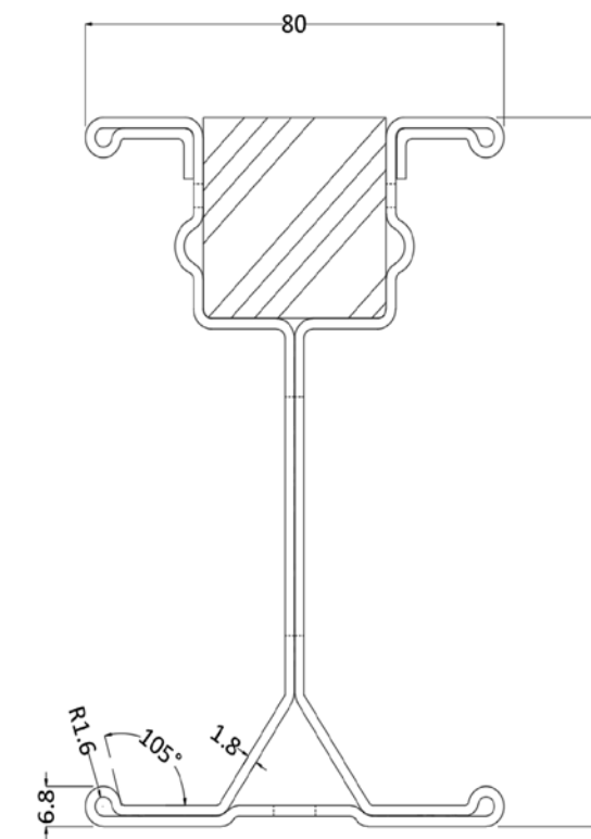
SMART WTD BEAM SECTION With 38x38 mm wood Nailing
